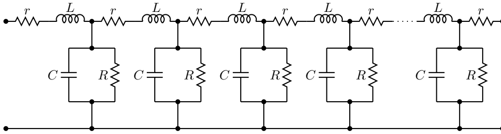
Figure 33: A lumped model of a transmission line, illustrating the use of custom macros.
