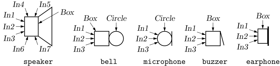
Figure 18: Audio components: speaker(U|D|L|R|degrees,size) , bell , microphone , buzzer , earphone , with their internally named positions and components.
