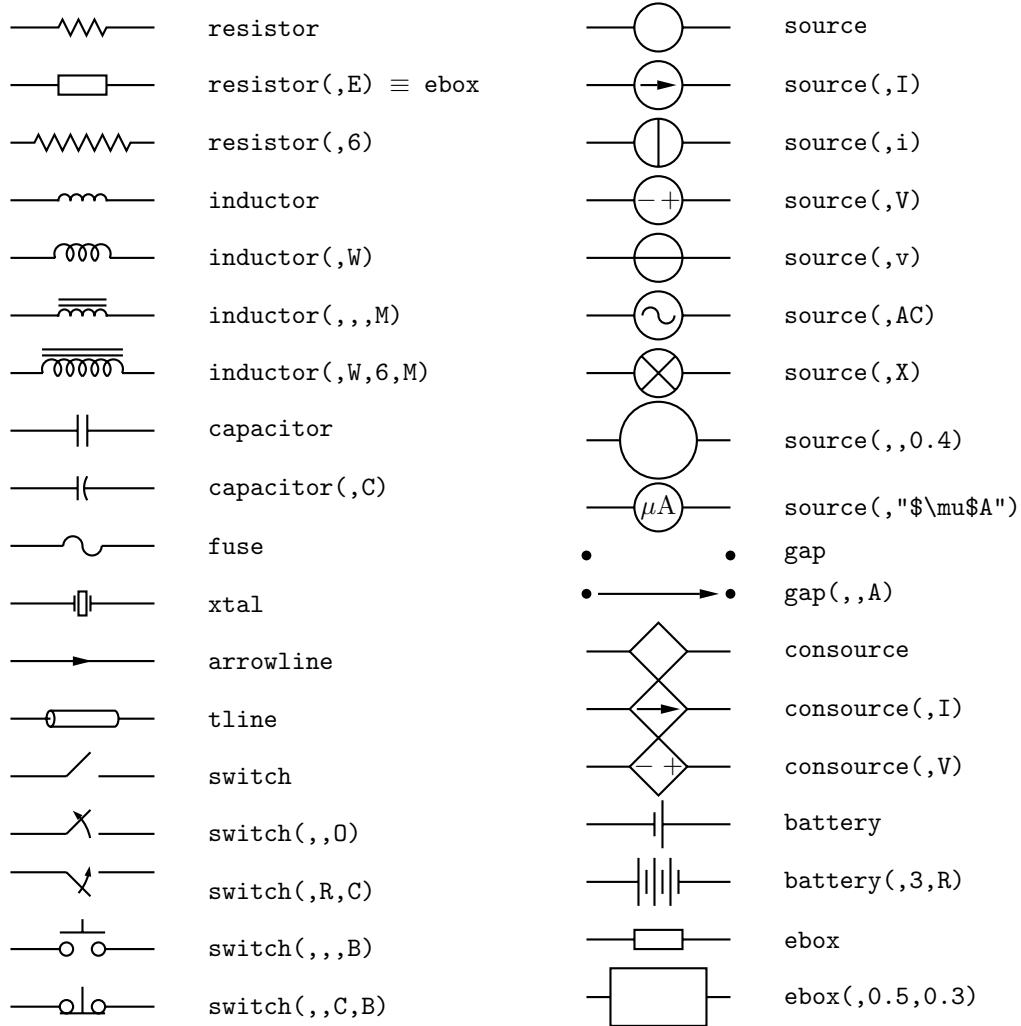
Figure 4: Two-terminal element macros, with some variations.
