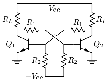
Figure 27: Bipolar transistor circuit, illustrating crossover.
