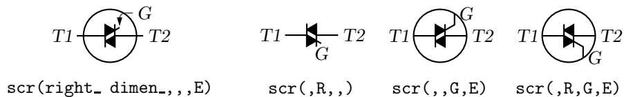
Figure 26: SCR elements, drawing direction to the right.
