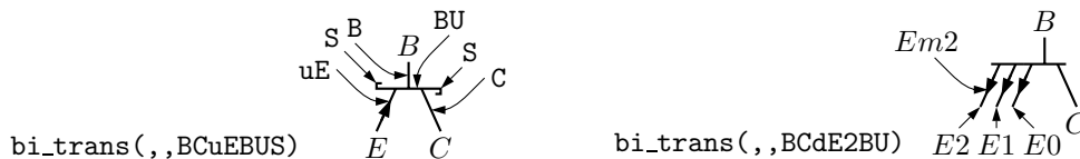
Figure 23: The bi_trans( linespec ,L|R, chars ,E) macro. The sub-elements are specified by the third argument. The substring En creates multiple emitters E0 to En .
