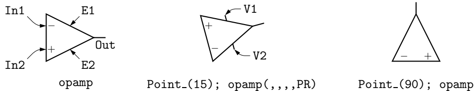
Figure 15: Operational amplifiers. The P option adds power connections. The second and third arguments can be used to place and rotate arbitrary text at In1 and In2 .
