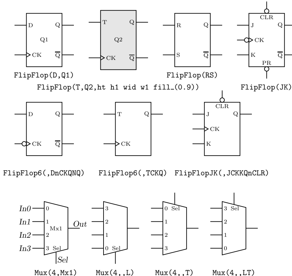
Figure 32: The FlipFlop and Mux macros, with variations.
