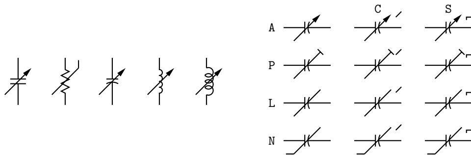
Figure 7: Illustrating variable('element', [A|P|L|[u]N] [C|S], angle, length) . For example, variable('capacitor(down_ dimen_) ' draws the leftmost capacitor shown above, and variable('resistor(down_ dimen_) ', uN) draws the resistor. The default angle is 45°, regardless of the direction of the element. The array on the right shows the effect of the second argument.
