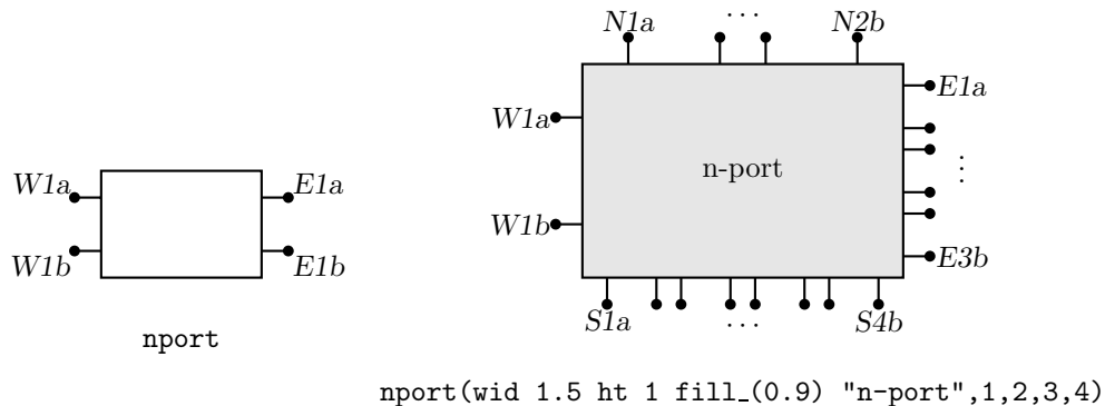
Figure 19: The nport macro draws a sequence of pairs of named pins on each side of a box. The default is a twoport. The pin names are shown.
