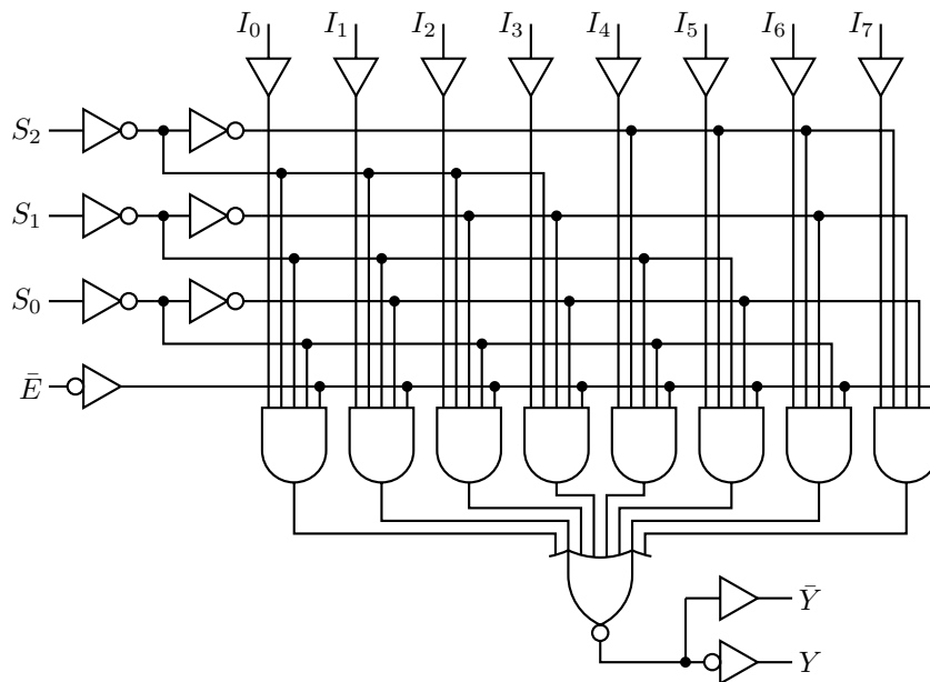
Figure 30: Eight-input binary multiplexer circuit, illustrating a gate with wings and for_ looping in the source.
