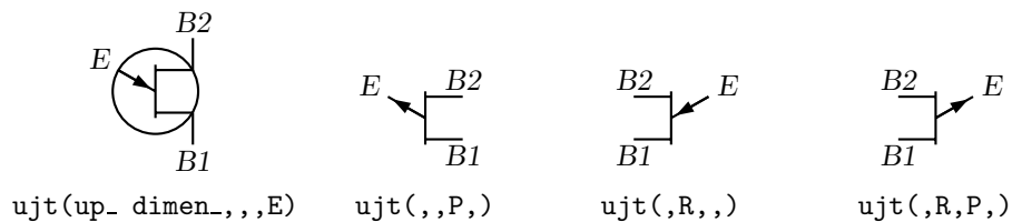
Figure 25: UJT devices, with current drawing direction up.
