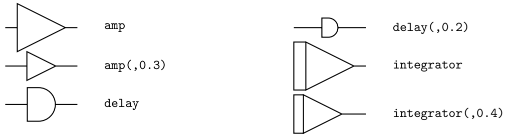
Figure 6: Amplifier, delay, and integrator.
