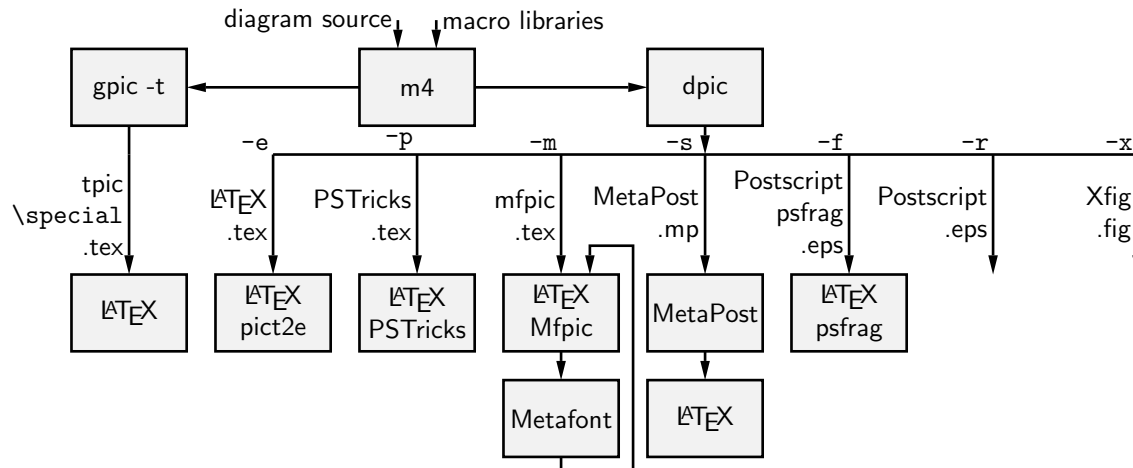
Figure 36: Output formats produced by gpic -t and dpic .
