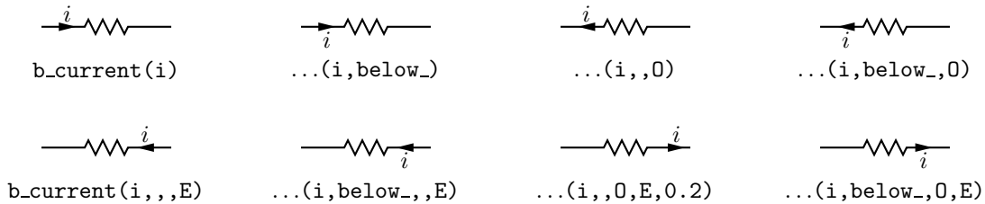
Figure 9: Illustrating b_current . In all cases the drawing direction is to the right.
