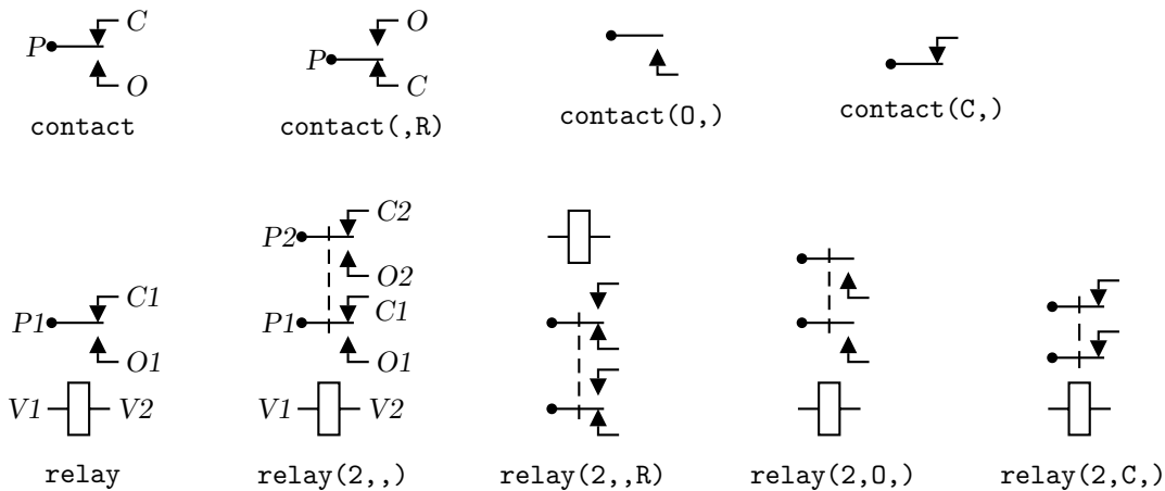
Figure 20: The contact and relay macros (default direction right).
