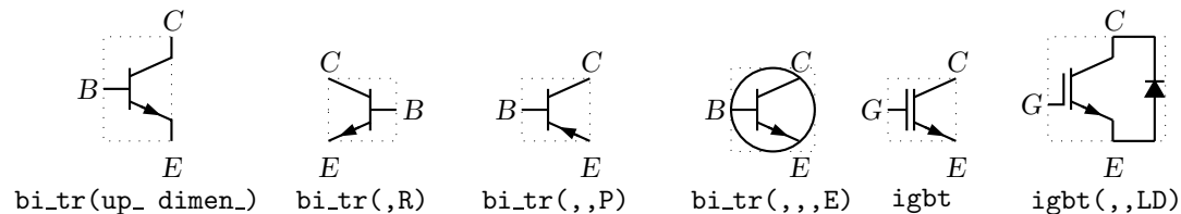
Figure 21: Bipolar transistor variants (current direction upward).
