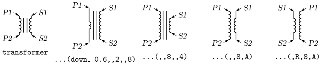
Figure 17: The transformer(linespec,L|R,np,A,ns) macro.
