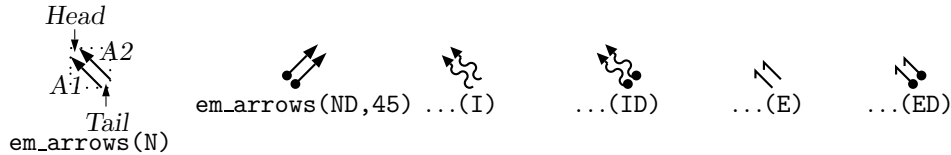
Figure 8: Radiation arrows: em_arrows(type, angle, length)
