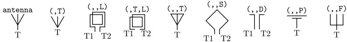
Figure 14: Antenna symbols, with macro arguments shown above and predefined terminal names below.
