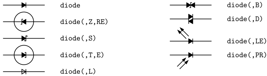
Figure 5: Variants of diode( linespec , B|D|L|LE[R]|P[R]|S|T|Z, [R] [E]) .
