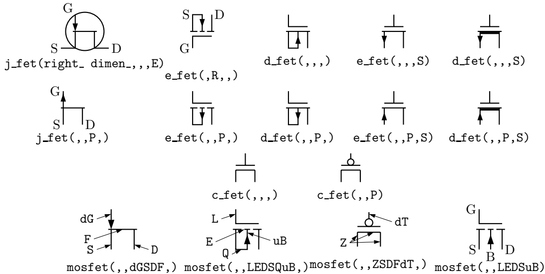
Figure 24: JFET, insulated-gate enhancement and depletion MOSFETS, and simplified versions, see [12]. These macros are wrappers that invoke the mosfet macro as shown in the bottom row. At the lower right is a custom device defined by omitting the substrate connection.
